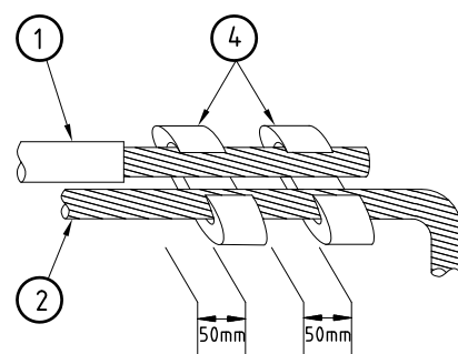
EARTHING CLAMPS - DETAIL B
