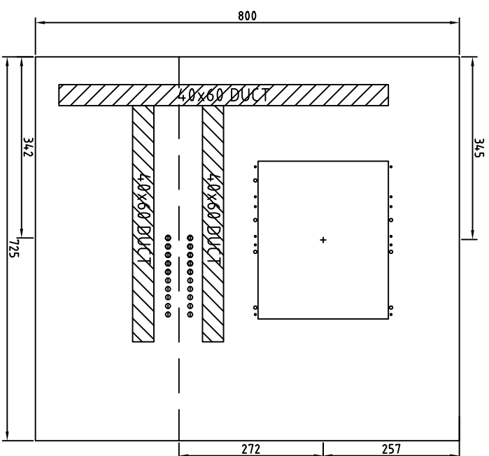
FRONT PANEL REAR VIEW DUCT & RAIL DETAILS
