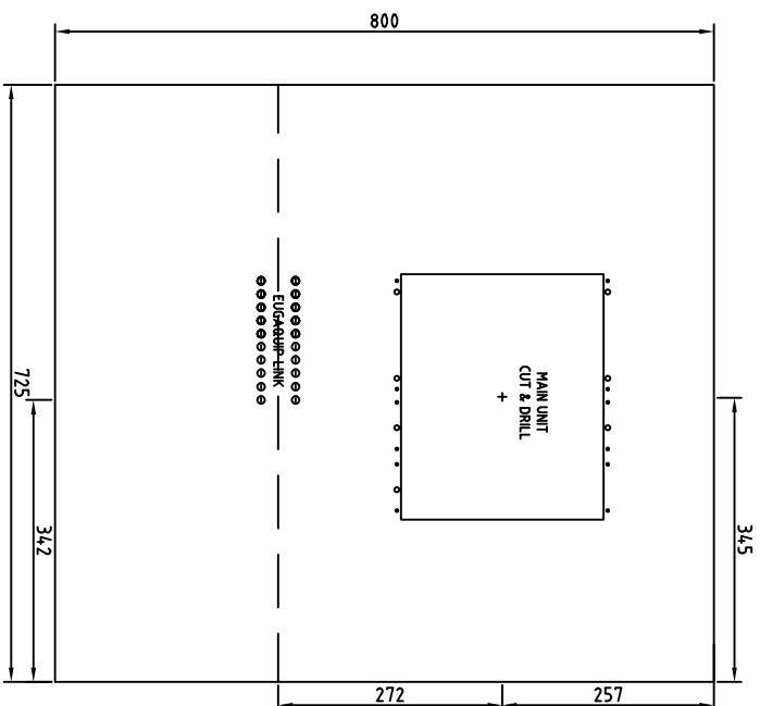
FRONT PANEL FRONT VIEW CUT & DRILL DETAILS
