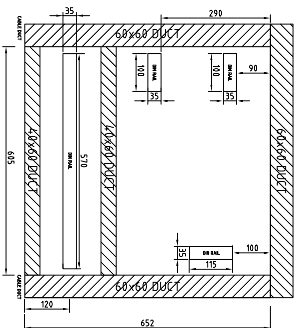
REAR MOUNTING PLATE INSIDE TRANSF CUBICLE
