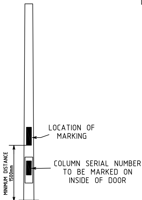
S/L COLUMN: (NOT TO SCALE)
