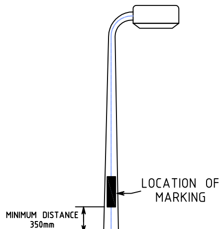
OUTREACH ARM (NOT TO SCALE)
