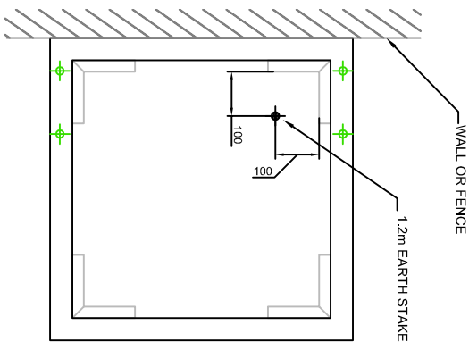
PLAN VIEW CUBICLE AND COVER OMITTED
